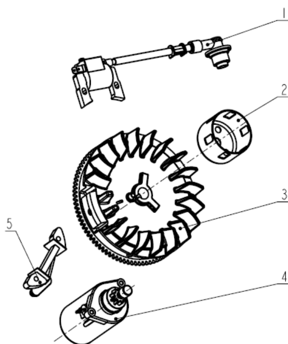
Ignition System Ass'y
