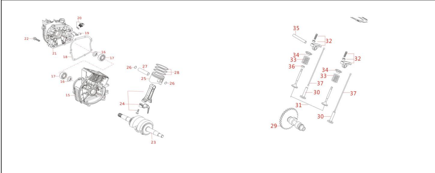
FIG.2 Crankcase Ass'y and piston Ass'y
