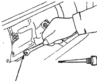
OIL DRAIN PLUG
